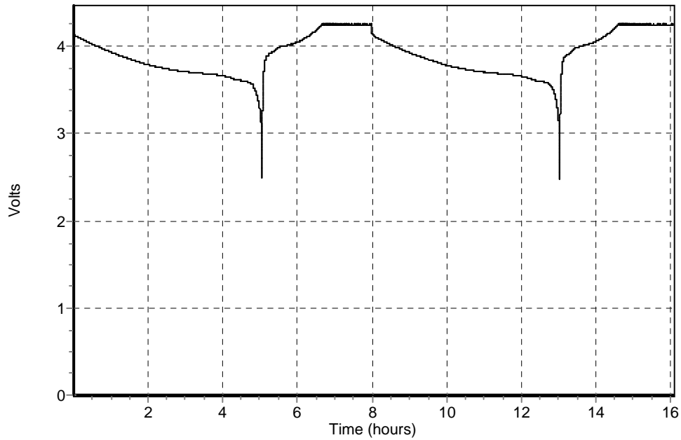
UBA4 Results File, Capacity: 1,737Ah.
