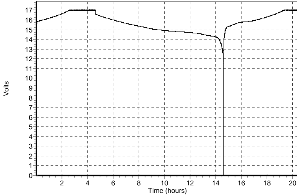
UBA4 Results File, Capacity: 10,51Ah.
